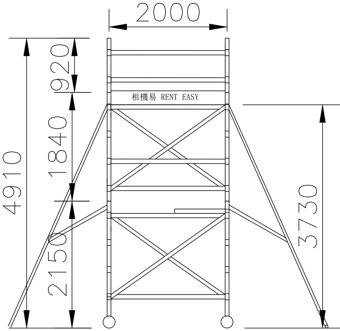
VIEW A
