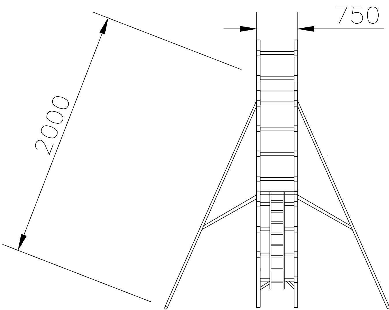
VIEW C
