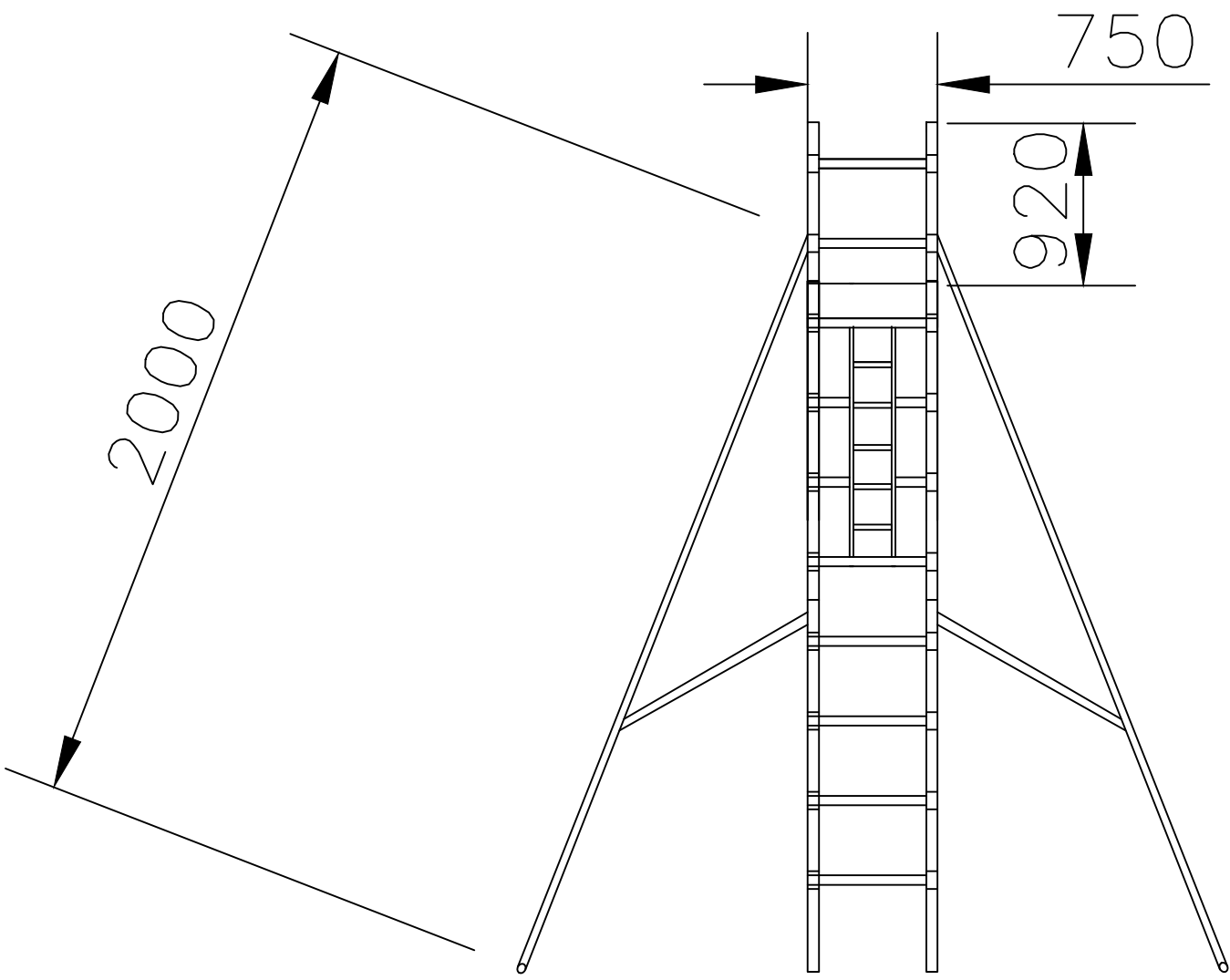
VIEW B
