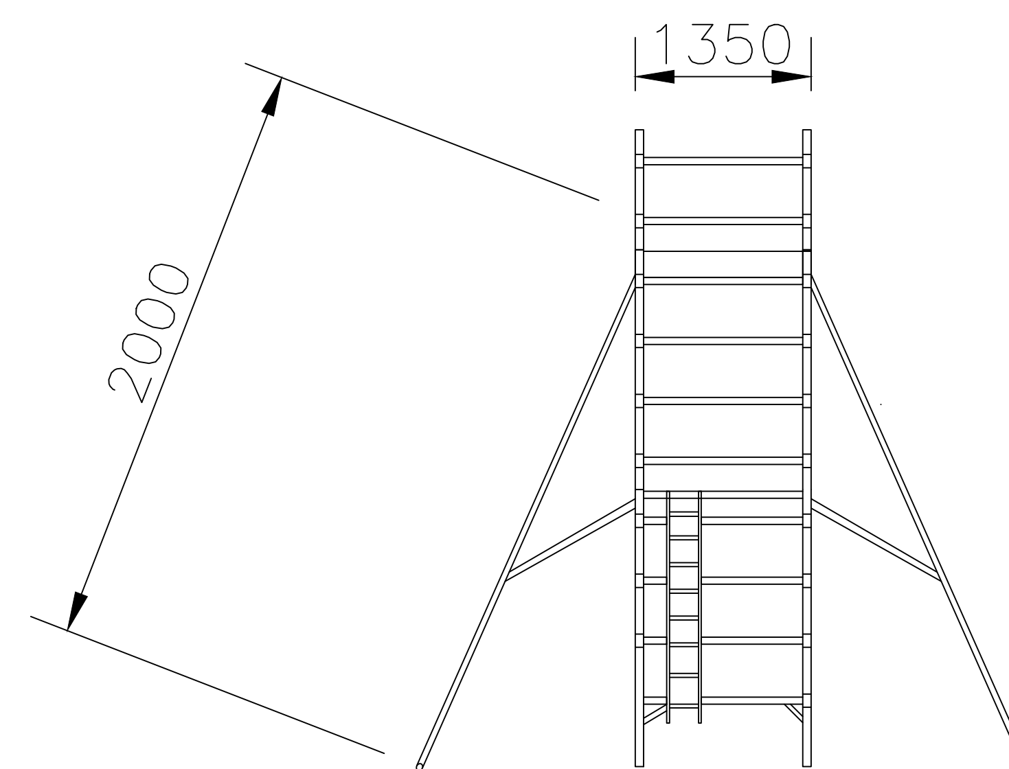
VIEW C
