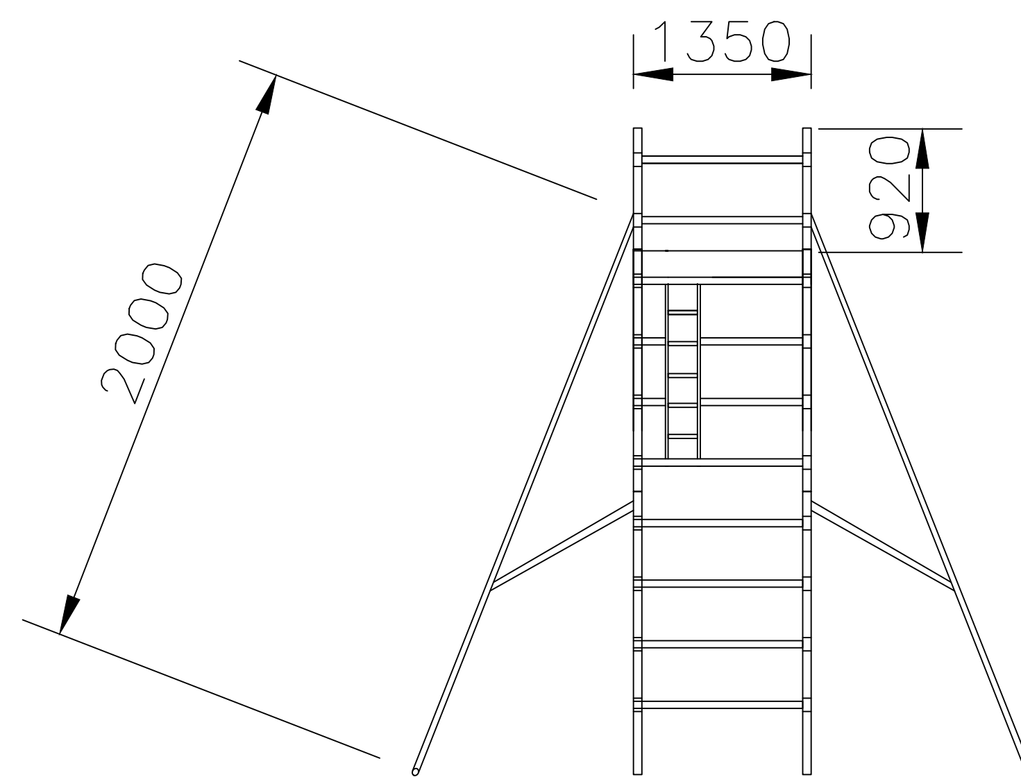
VIEW B
