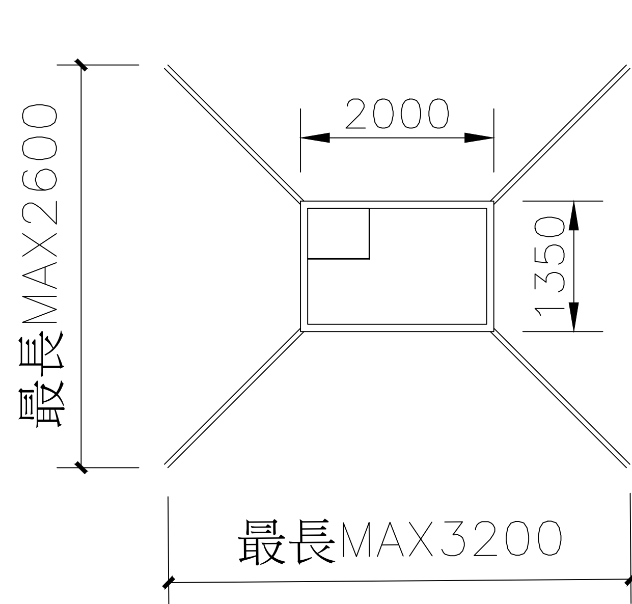
VIEW D
