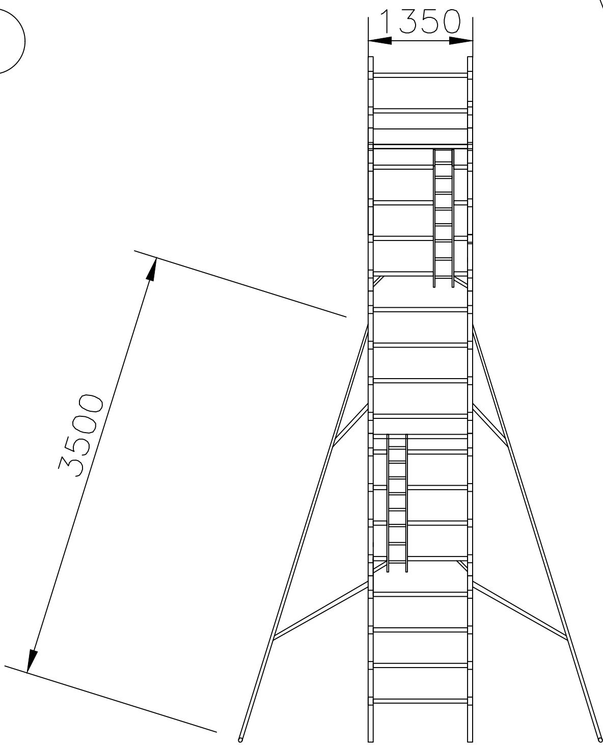
VIEW B
