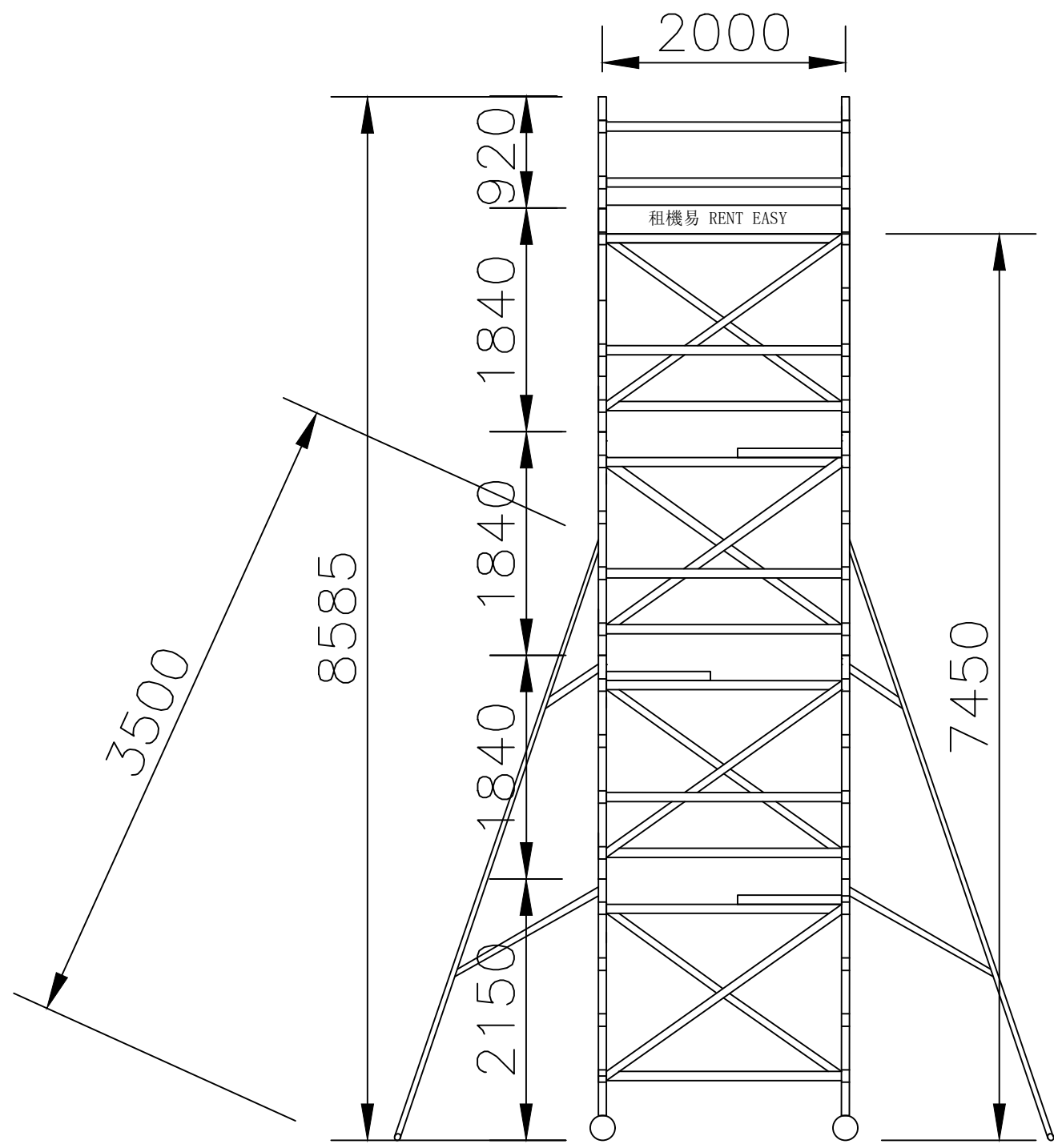
VIEW A
