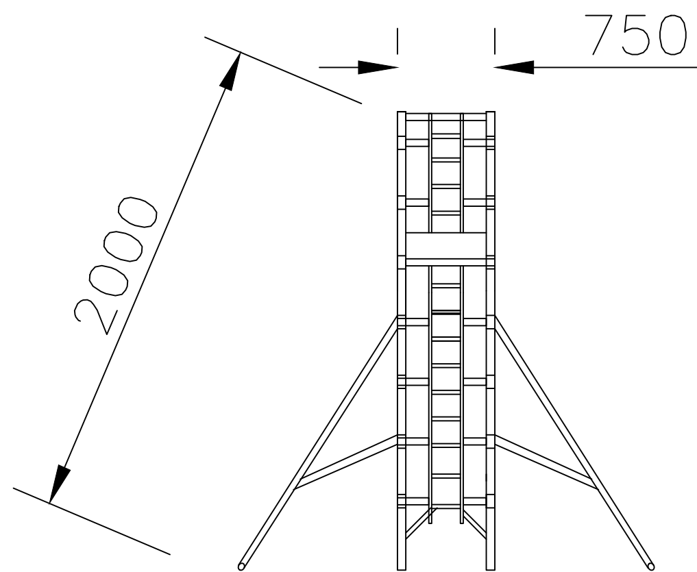
VIEW C
