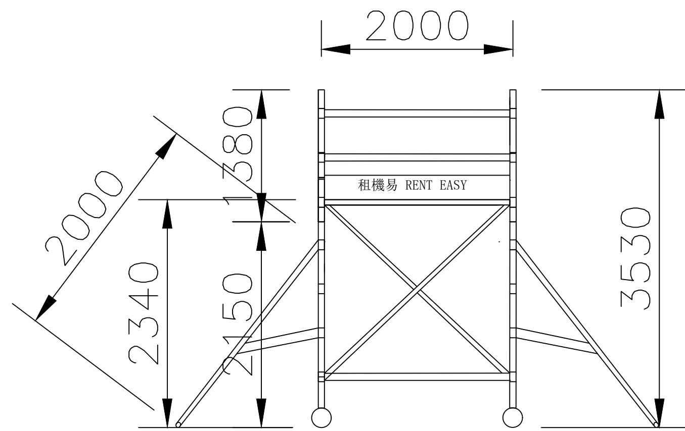
VIEW A
