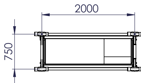
VIEW C
