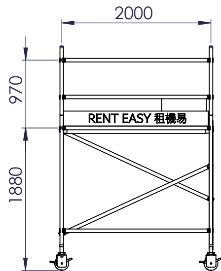
VIEW A
