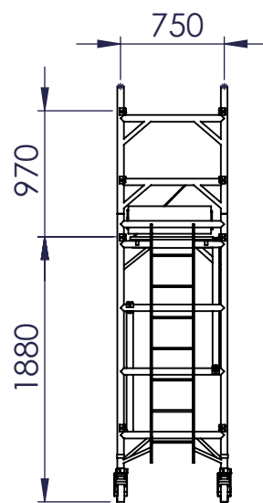
VIEW B
