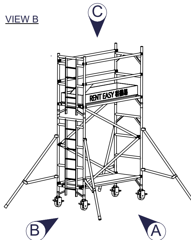
ISO VIEW
