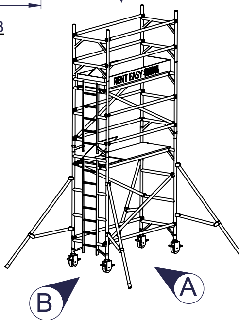
ISO VIEW
