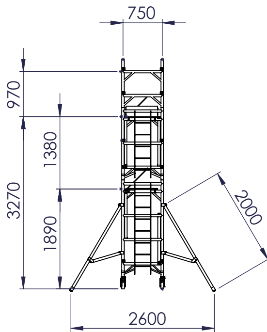
VIEW B
