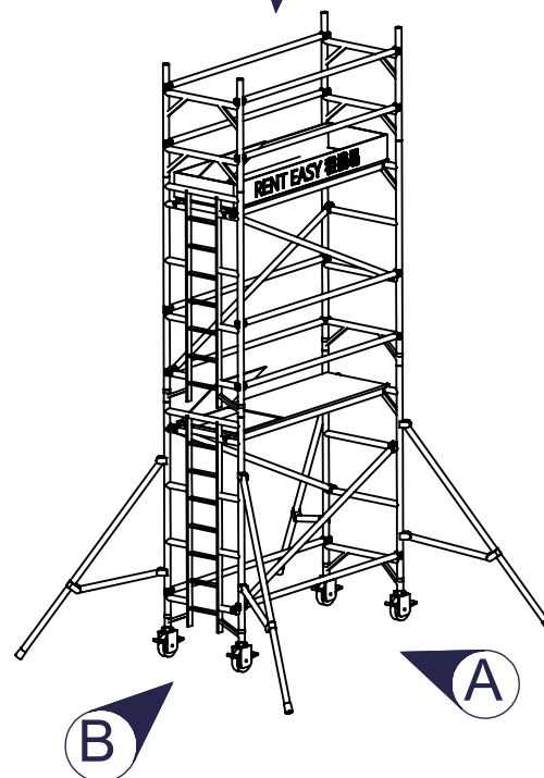
ISO VIEW
