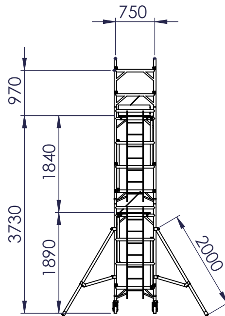
VIEW B
