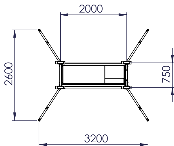
VIEW C
