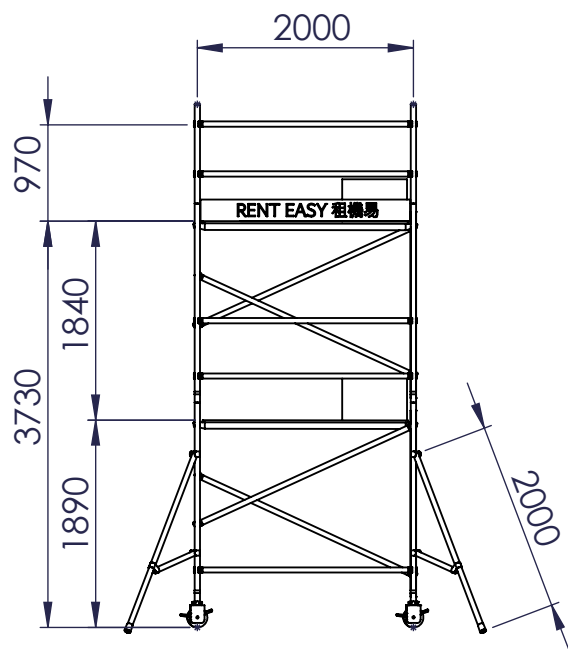
VIEW A
